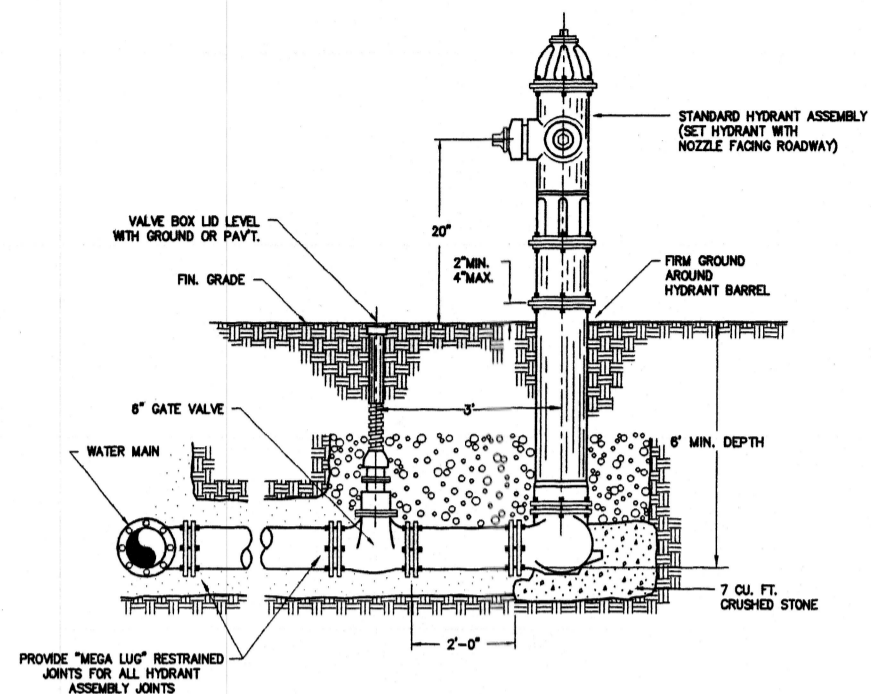
DETAIL-HYDRANT INSTALLATION NO SCALE
