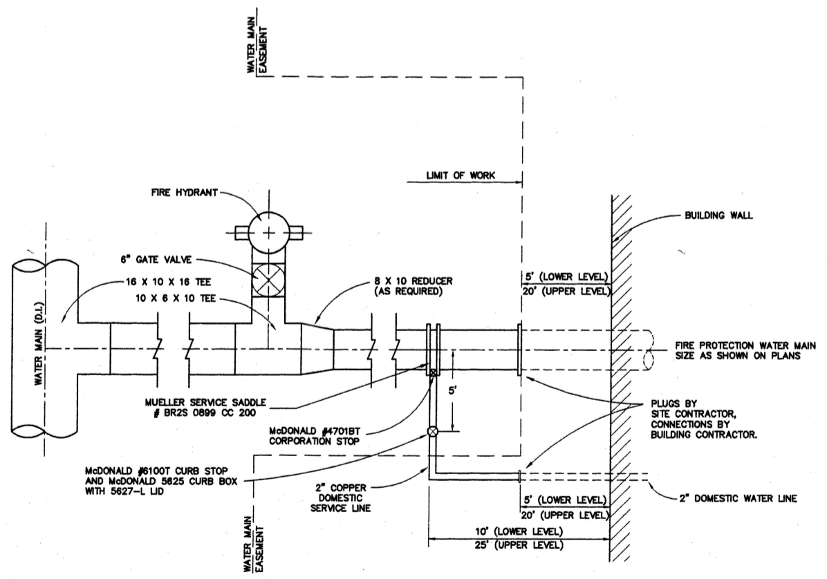
WATER SERVICE LINE DETAIL NO SCALE
