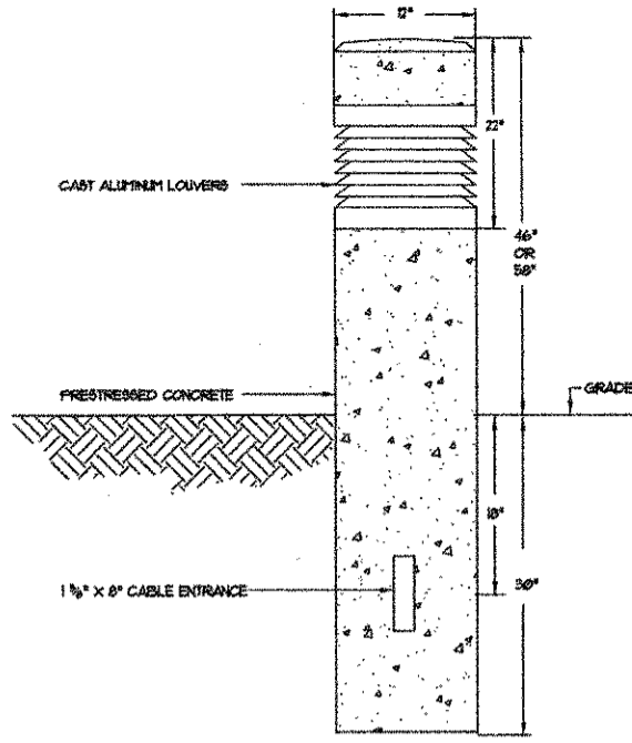
ALTERNATE DECORATIVE BOLLARD - "N01" SCALE 1/8"
