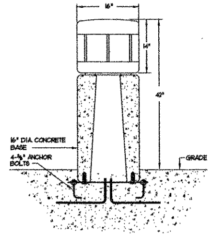
DECORATIVE BOLLARD - "BA" SCALE 1/4"
